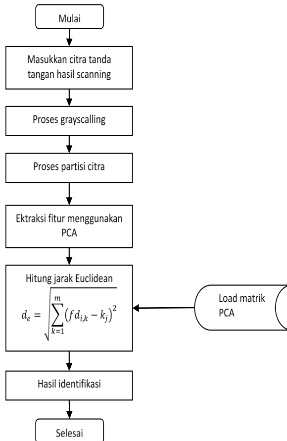
Gambar 5. Alur data testing
