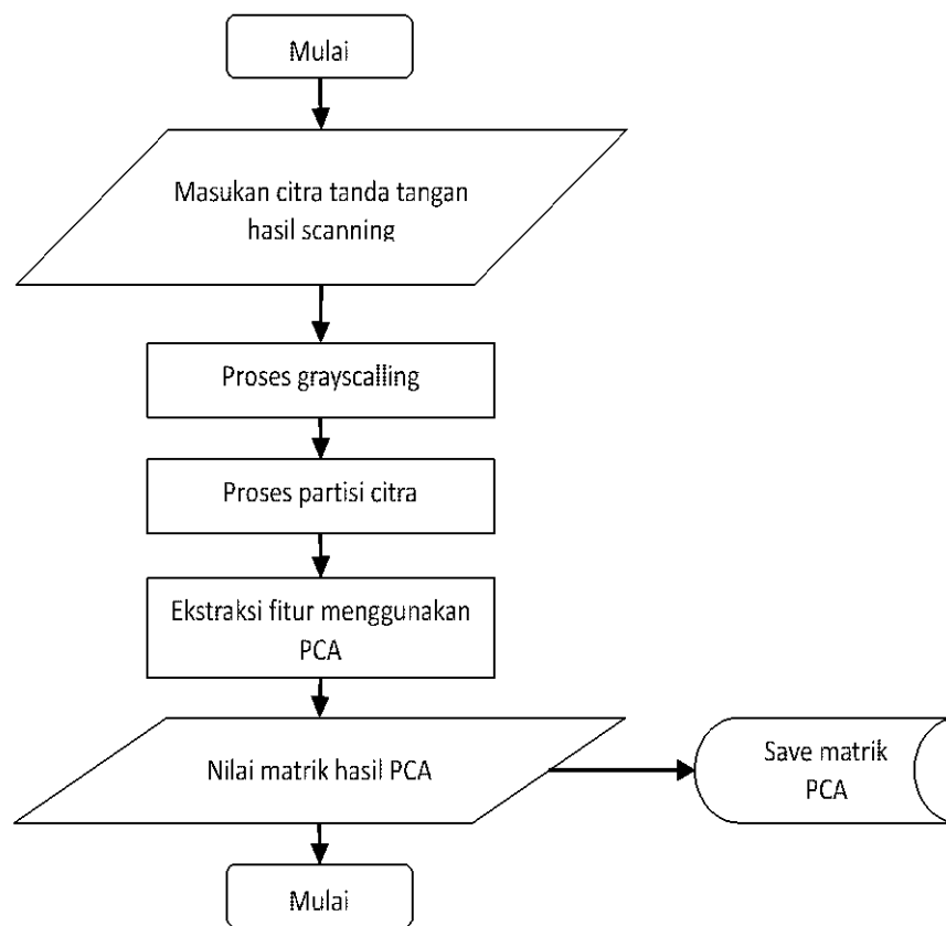
Gambar 4. Alur data training
