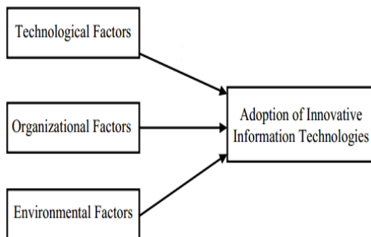
Gambar 1. TOE Framework
