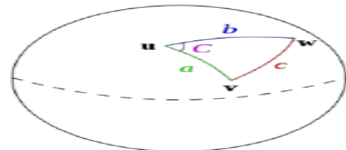
Figure 4. Haversine Method [6]
