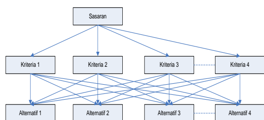
Gambar 3. Analytical Hierarchy Process.
